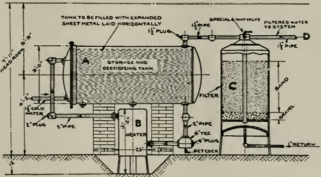
THE PROPOSED SYSTEM FOR PREVENTING CORROSION OF WATER PIPES
